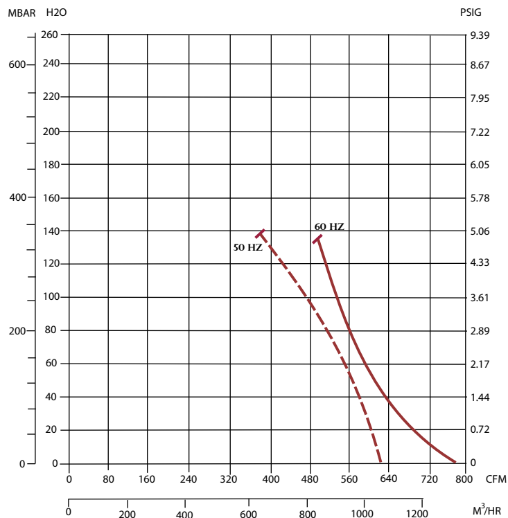
Vacuum vs. CFM
