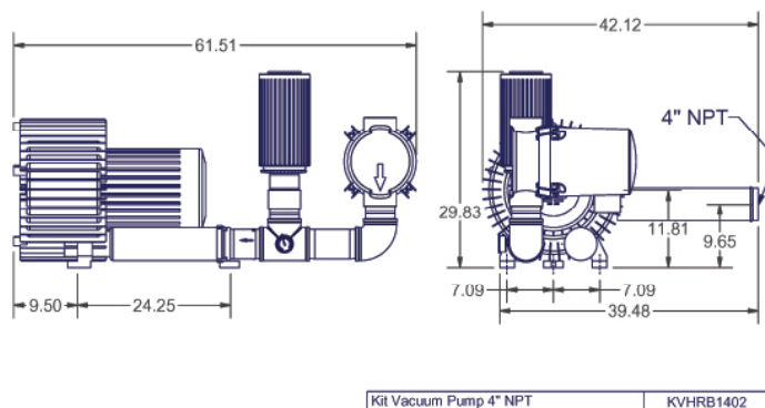
KVHRB1402 - Vacuum Kit Drawing
