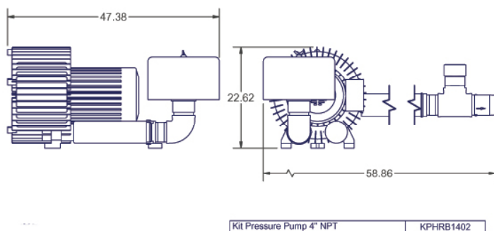
KPHRB1402 - Pressure Kit Drawing
