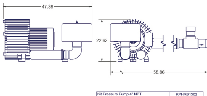
KPHRB1302 - Pressure Kit Drawing
