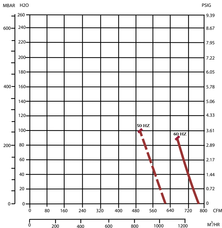
Pressure vs. CFM
