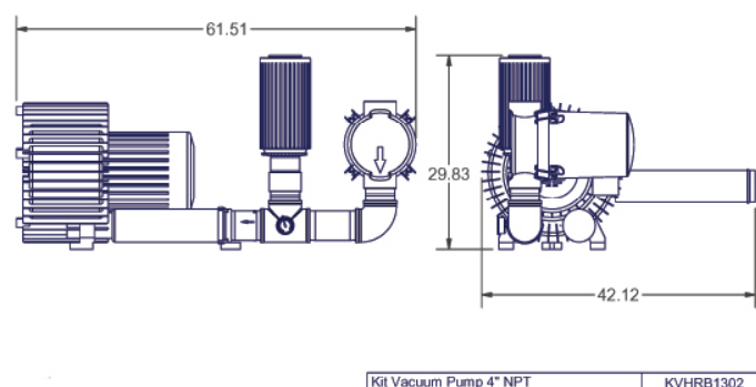
KVHRB1302 - Vacuum Kit Drawing
